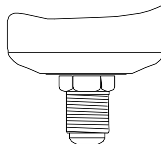
Fig. 6 Style 5 7/16-20 UNF
